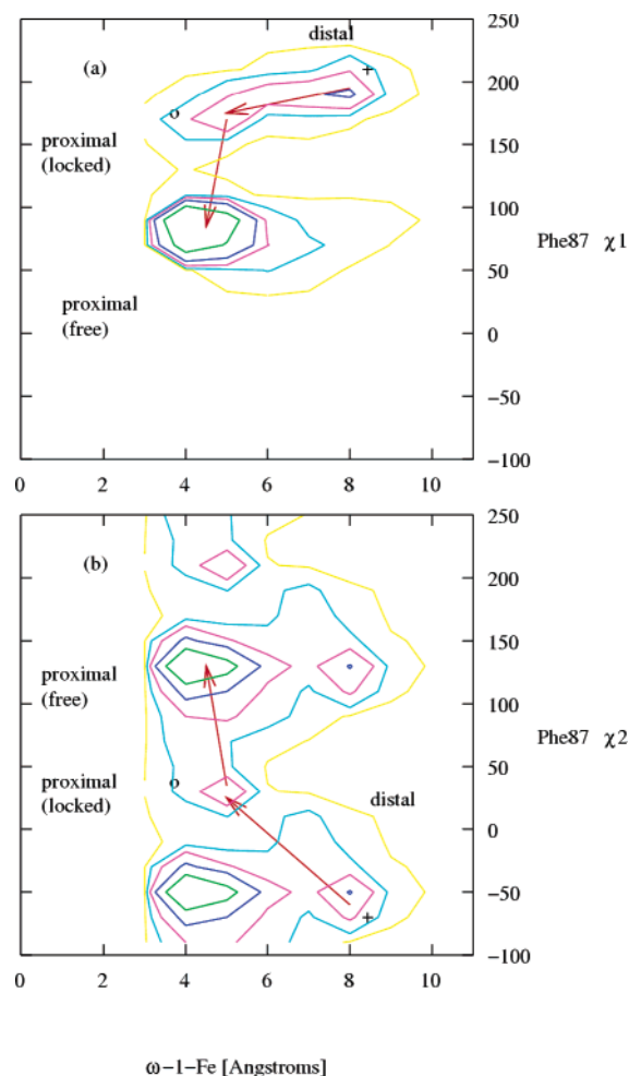
Figure 5. The population distributions at 302 K of P450 BM-3/NPG conformations as a function of (a) the \omega-1-Fe distance and the \chi_1 angle of Phe87 and (b) the \omega-1-Fe distance and the \chi_2 angle of Phe87. The coordinates corresponding to the X-ray crystal conformation and the proximal state conformation predicted by Jovanovic et al. are indicated by a cross and a circle, respectively. The distal state, the proximal locked ligand, and proximal free ligand states are indicated. Contours are drawn at 1 \times 10^{-3} , 1 \times 10^{-2} , 2.5 \times 10^{-2} , 5 \times 10^{-2} , and 1 \times 10^{-1} fractional population.
