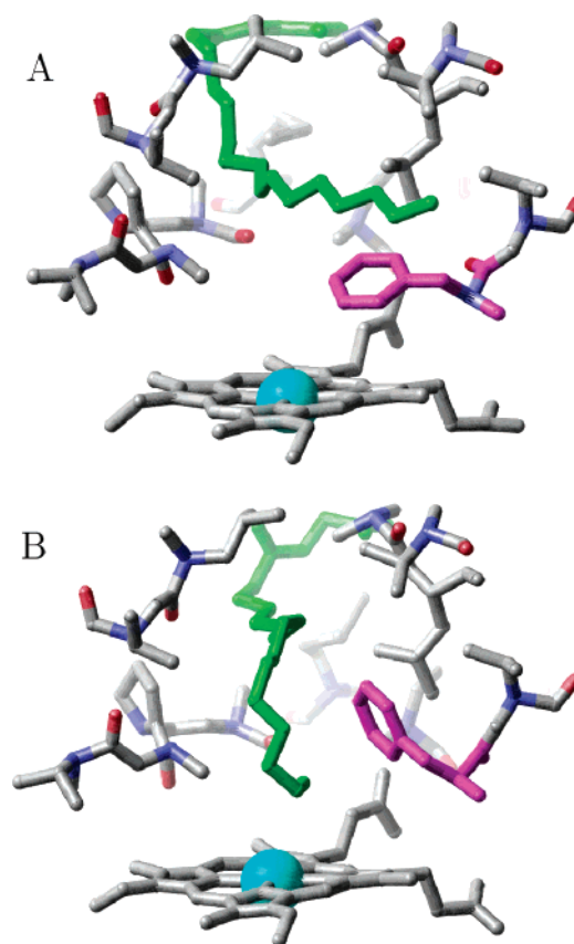
Figure 1. Active site of the P450 BM-3/NPG complex in (a) the low temperature X-ray conformation (PDB 1j pz) representative of distal state where the NPG (shown in green) is distant from the heme iron, with Phe87 (shown in magenta) interposed between NPG and heme iron (shown in blue) and (b) the alternative active site of the conformation predicted by Jovanovic et al. representative of the proximal state where Phe87 has changed its rotameric state to allow NPG to approach the heme iron.
